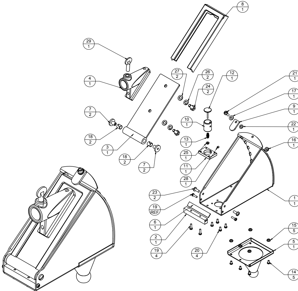
ISOMETRIC VIEW
